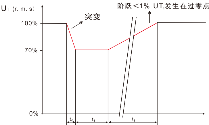
电压暂降、短时中断和电压变化 / Dips , Interruptions & Variations
